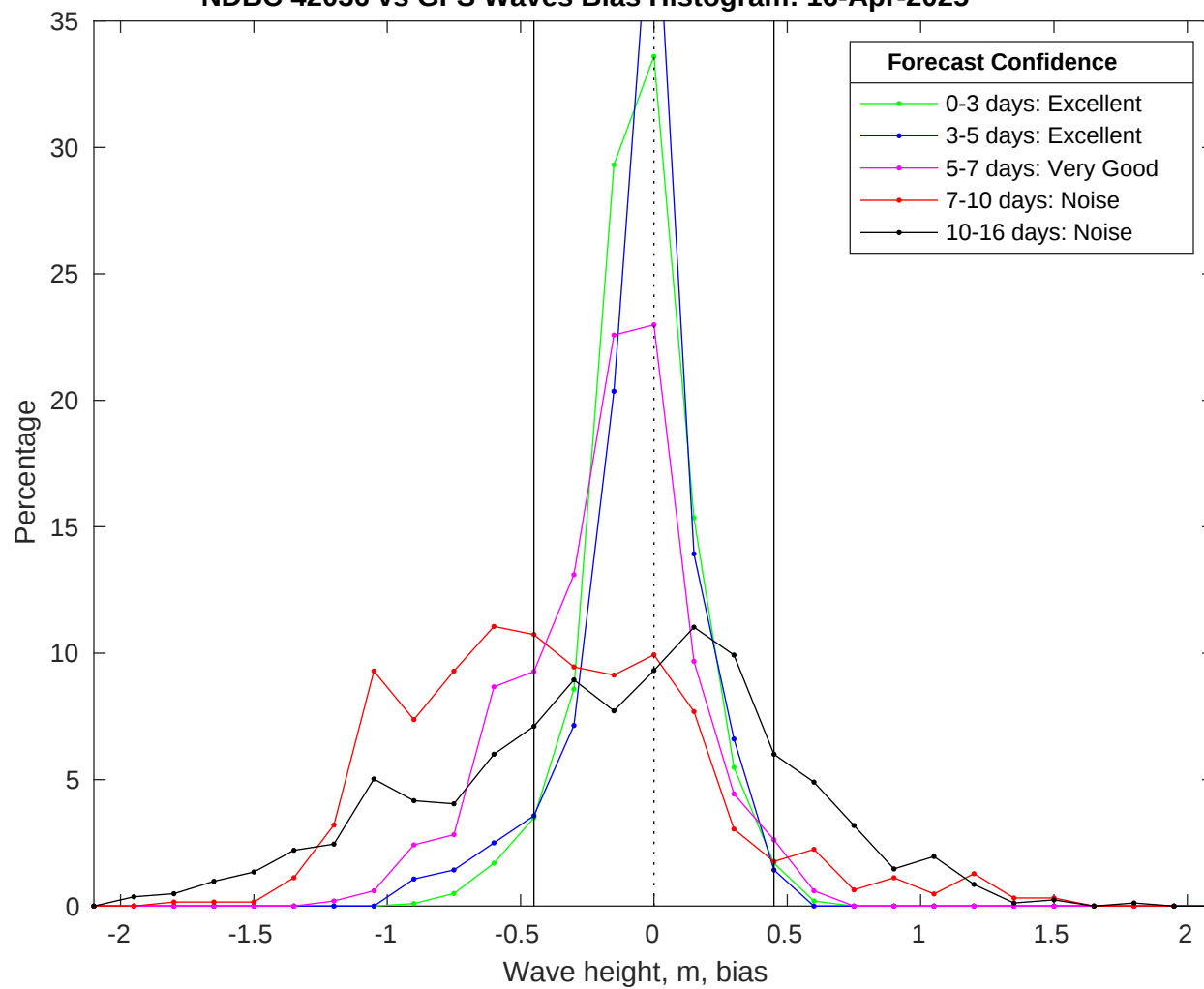
NDBC 42036 vs GFS Waves Bias Histogram: 16-Apr-2025
