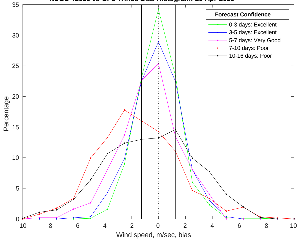
NDBC 42036 vs GFS Winds Bias Histogram: 16-Apr-2025
