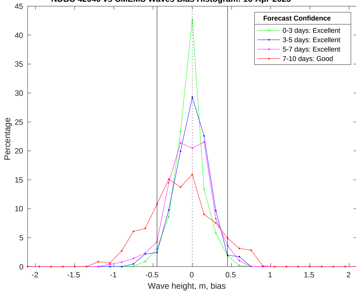
NDBC 42040 vs CMEMS Waves Bias Histogram: 16-Apr-2025
