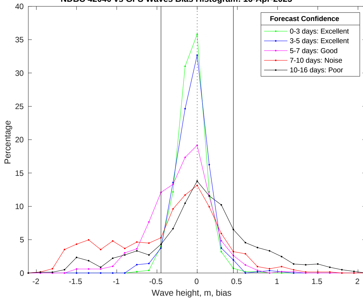
NDBC 42040 vs GFS Waves Bias Histogram: 16-Apr-2025
