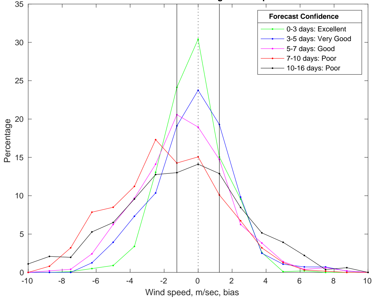
NDBC 42040 vs GFS Winds Bias Histogram: 16-Apr-2025
