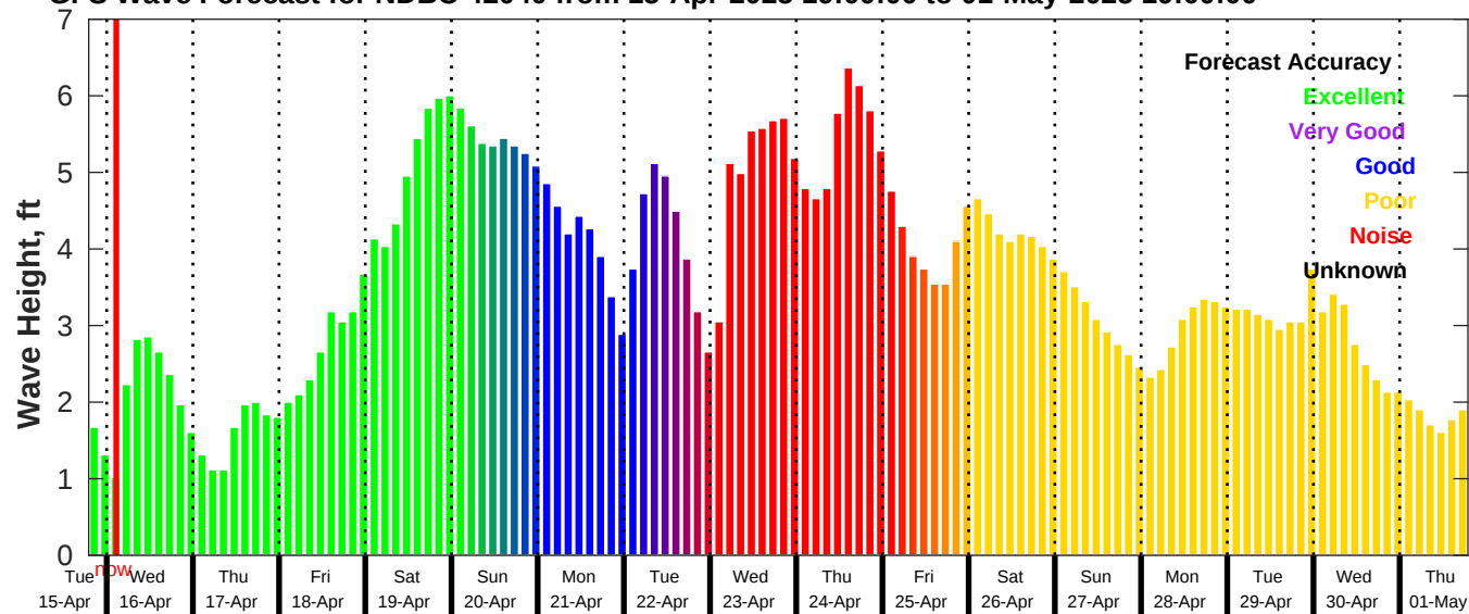
GFS Wave Forecast for NDBC 42040 from 15-Apr-2025 19:00:00 to 01-May-2025 19:00:00
