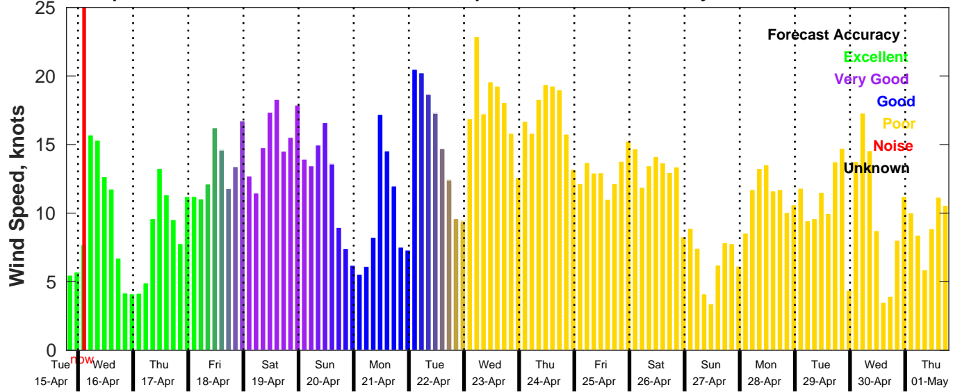
GFS Wind Speed Forecast for NDBC 42040 from 15-Apr-2025 19:00:00 to 01-May-2025 19:00:00
