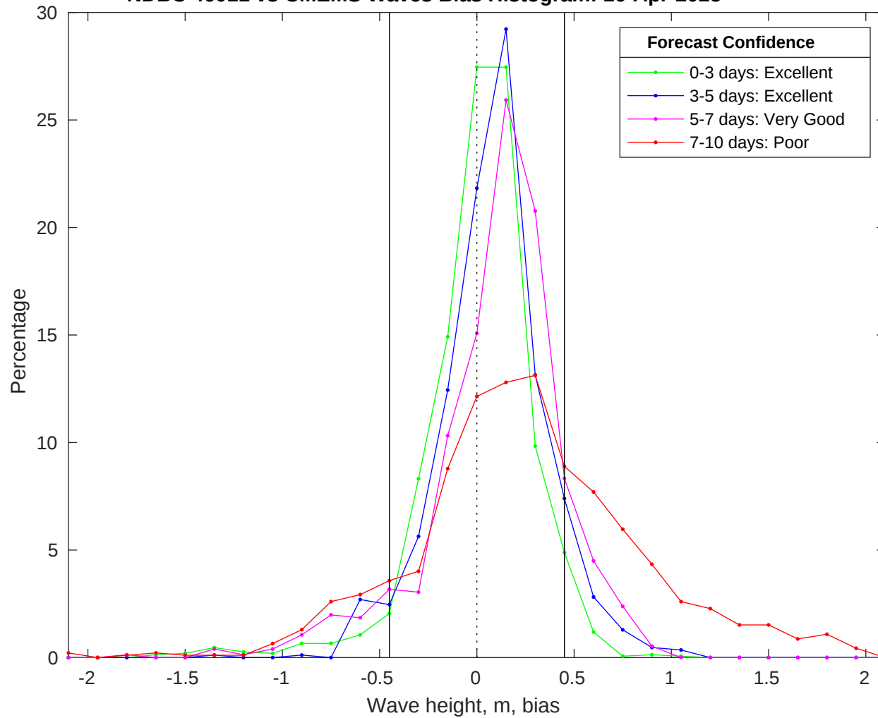
NDBC 46011 vs CMEMS Waves Bias Histogram: 16-Apr-2025
