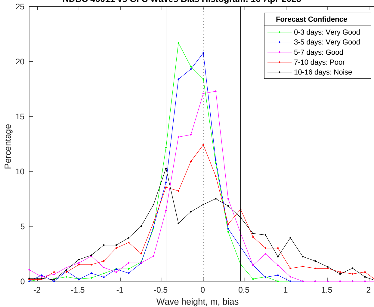
NDBC 46011 vs GFS Waves Bias Histogram: 16-Apr-2025
