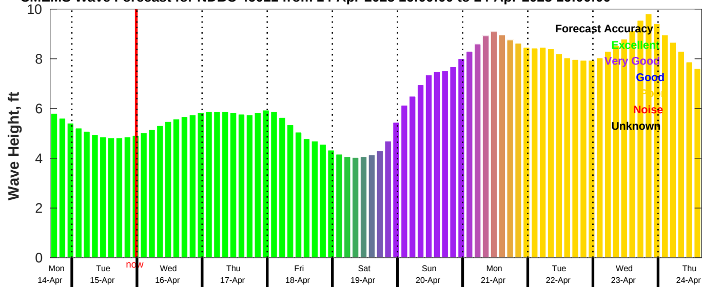
CMEMS Wave Forecast for NDBC 46011 from 14-Apr-2025 16:00:00 to 24-Apr-2025 16:00:00
