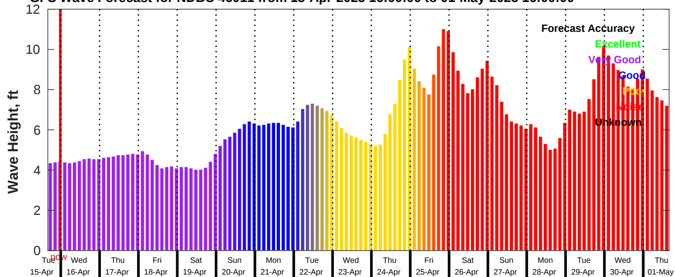
GFS Wave Forecast for NDBC 46011 from 15-Apr-2025 16:00:00 to 01-May-2025 16:00:00
