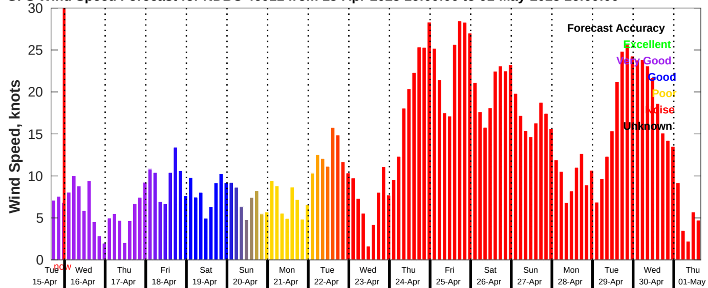
GFS Wind Speed Forecast for NDBC 46011 from 15-Apr-2025 16:00:00 to 01-May-2025 16:00:00
