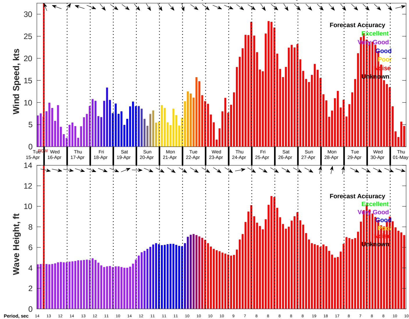
Wind & Wave Forecast for NDBC 46011 from 15-Apr-2025 16:00:00 to 01-May-2025 16:00:00
