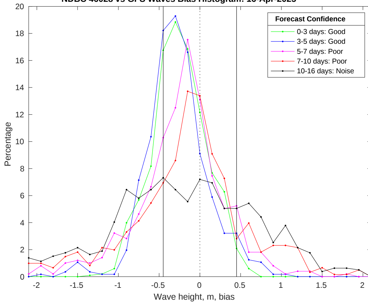
NDBC 46028 vs GFS Waves Bias Histogram: 16-Apr-2025
