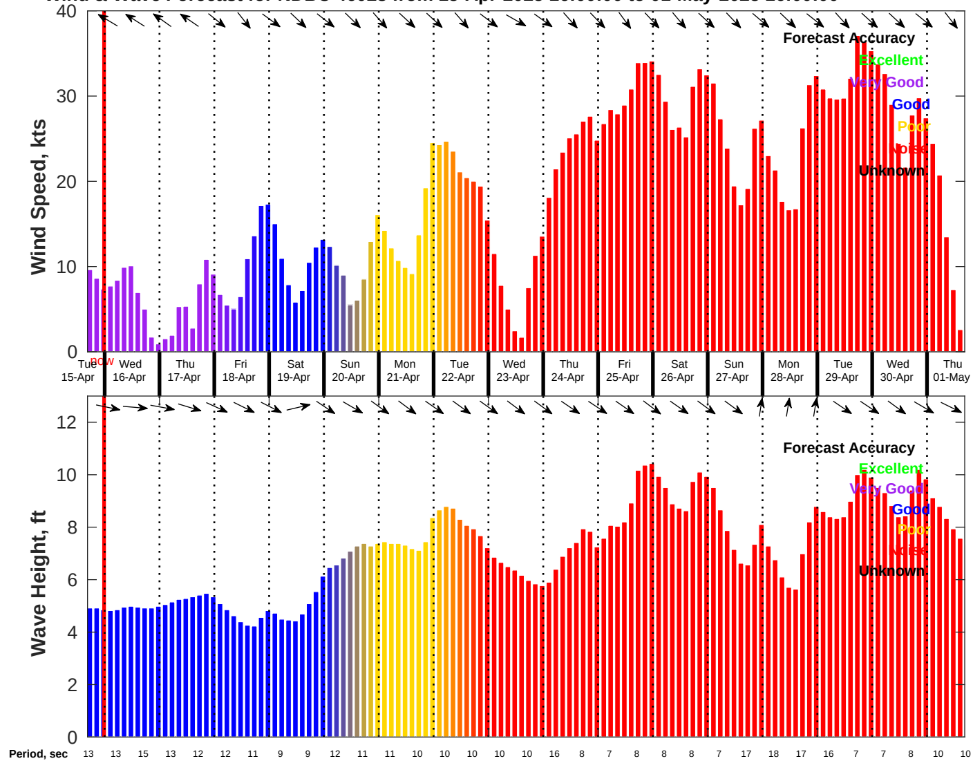
Wind & Wave Forecast for NDBC 46028 from 15-Apr-2025 16:00:00 to 01-May-2025 16:00:00
