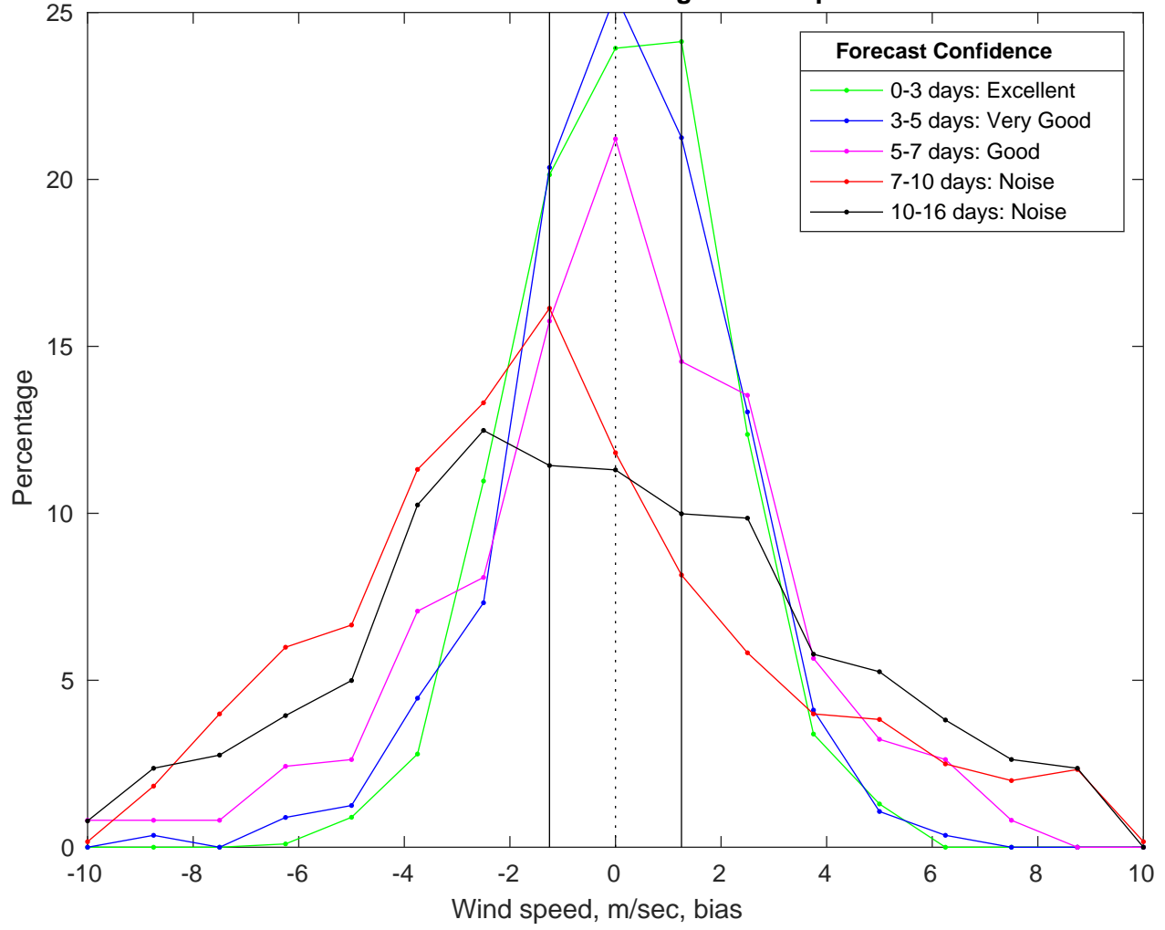
NDBC 46054 vs GFS Winds Bias Histogram: 16-Apr-2025
