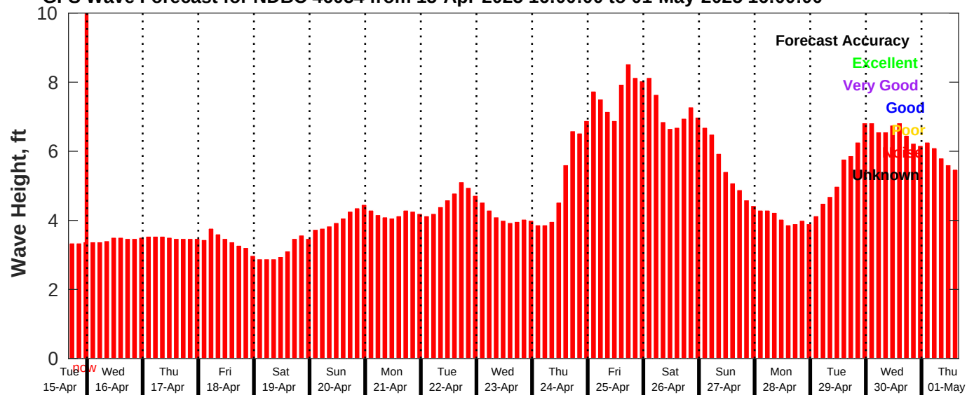
GFS Wave Forecast for NDBC 46054 from 15-Apr-2025 16:00:00 to 01-May-2025 16:00:00
