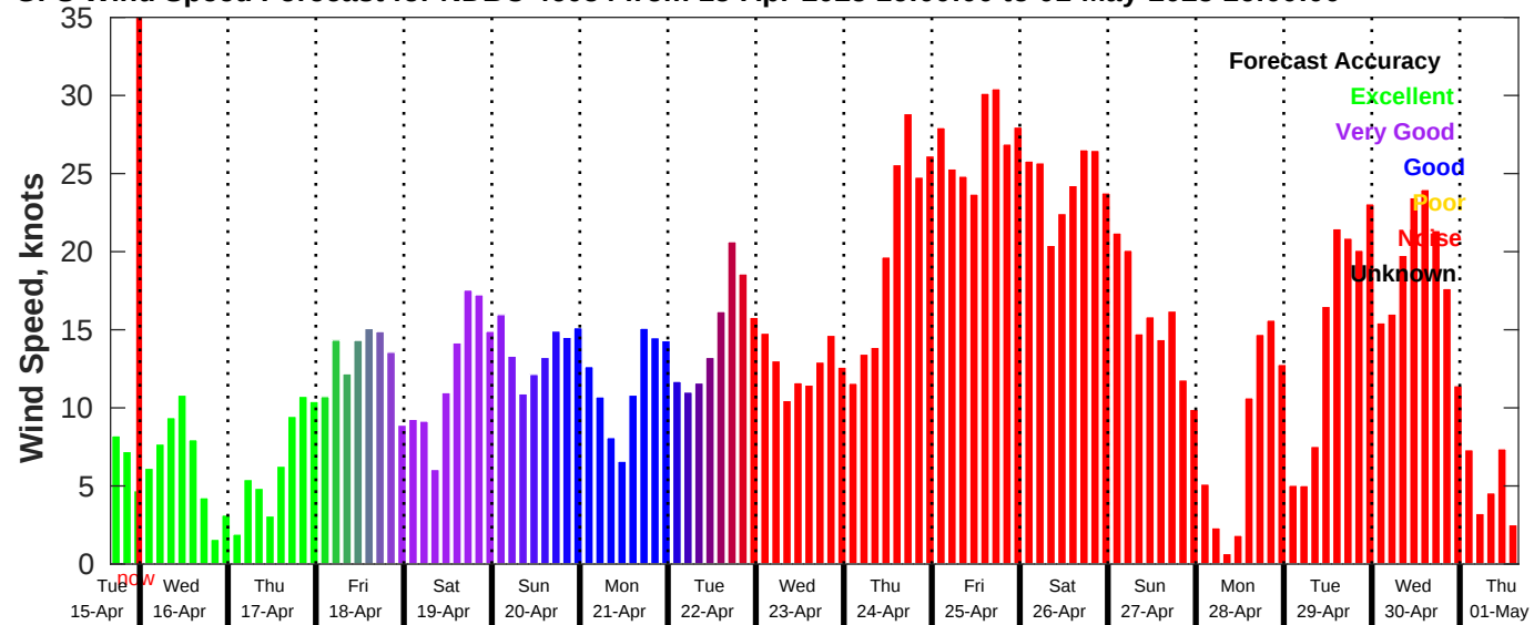
GFS Wind Speed Forecast for NDBC 46054 from 15-Apr-2025 16:00:00 to 01-May-2025 16:00:00
