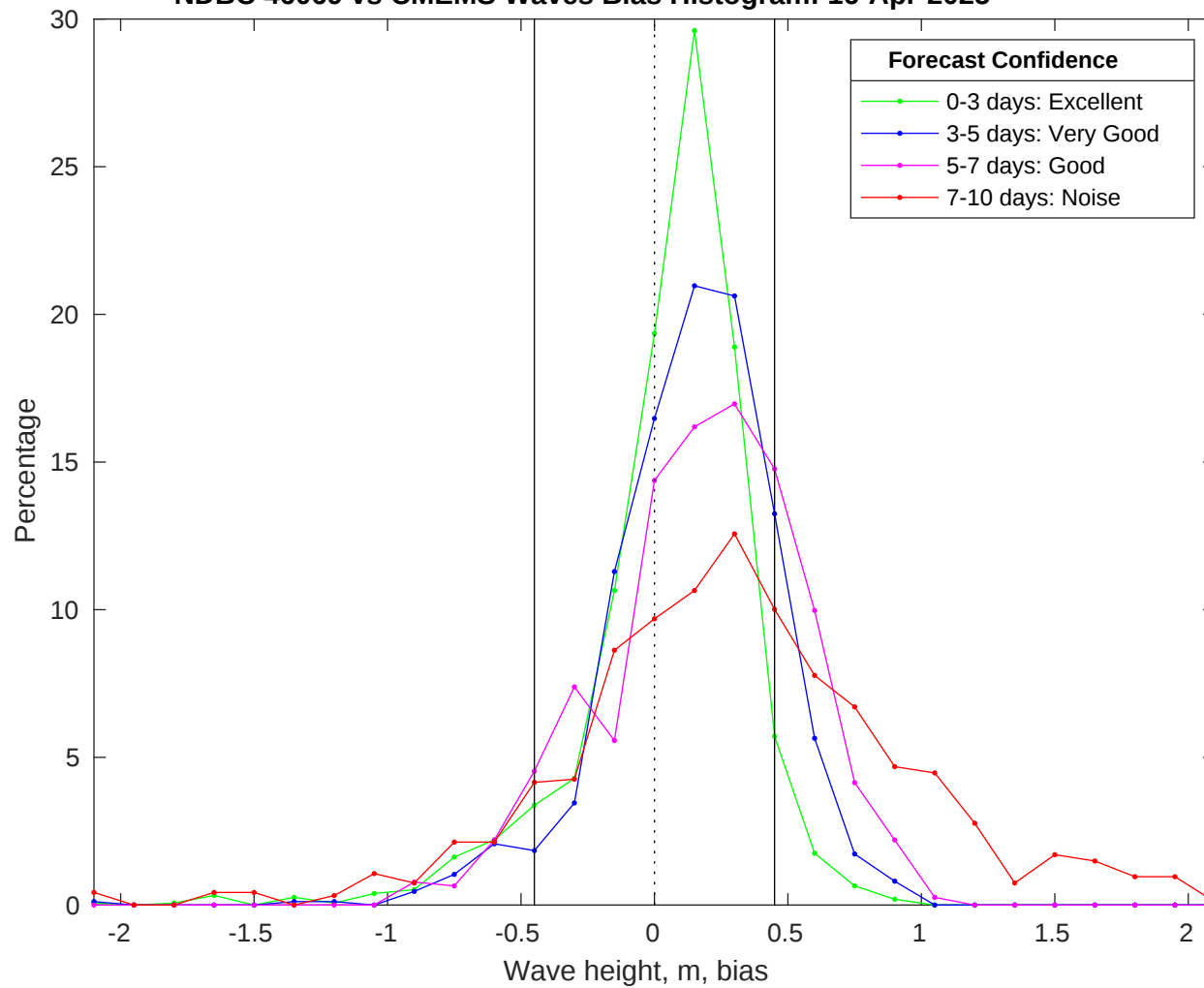
NDBC 46069 vs CMEMS Waves Bias Histogram: 16-Apr-2025
