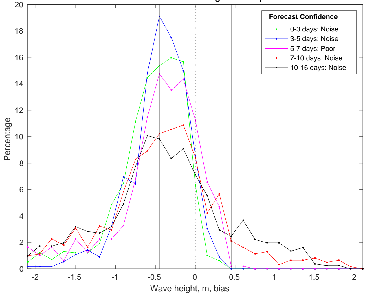
NDBC 46069 vs GFS Waves Bias Histogram: 16-Apr-2025
