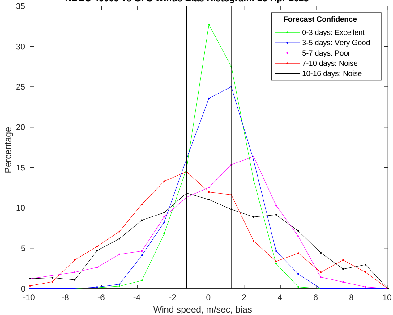
NDBC 46069 vs GFS Winds Bias Histogram: 16-Apr-2025
