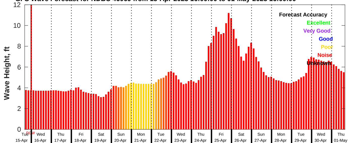
GFS Wave Forecast for NDBC 46069 from 15-Apr-2025 16:00:00 to 01-May-2025 16:00:00
