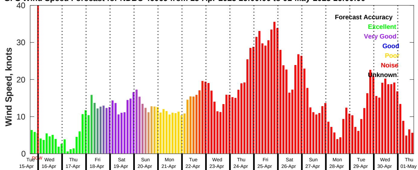
GFS Wind Speed Forecast for NDBC 46069 from 15-Apr-2025 16:00:00 to 01-May-2025 16:00:00
