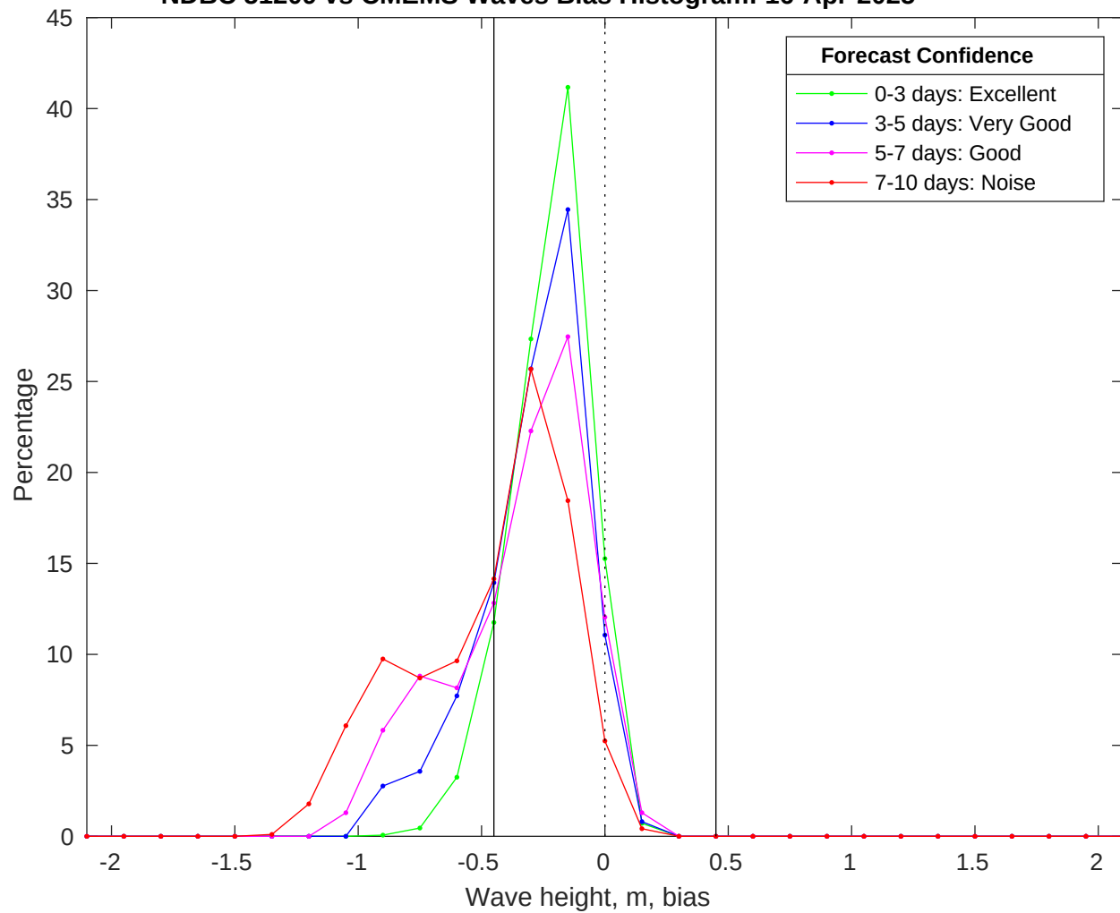
NDBC 51209 vs CMEMS Waves Bias Histogram: 16-Apr-2025
