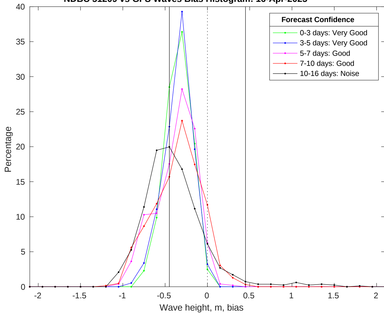
NDBC 51209 vs GFS Waves Bias Histogram: 16-Apr-2025
