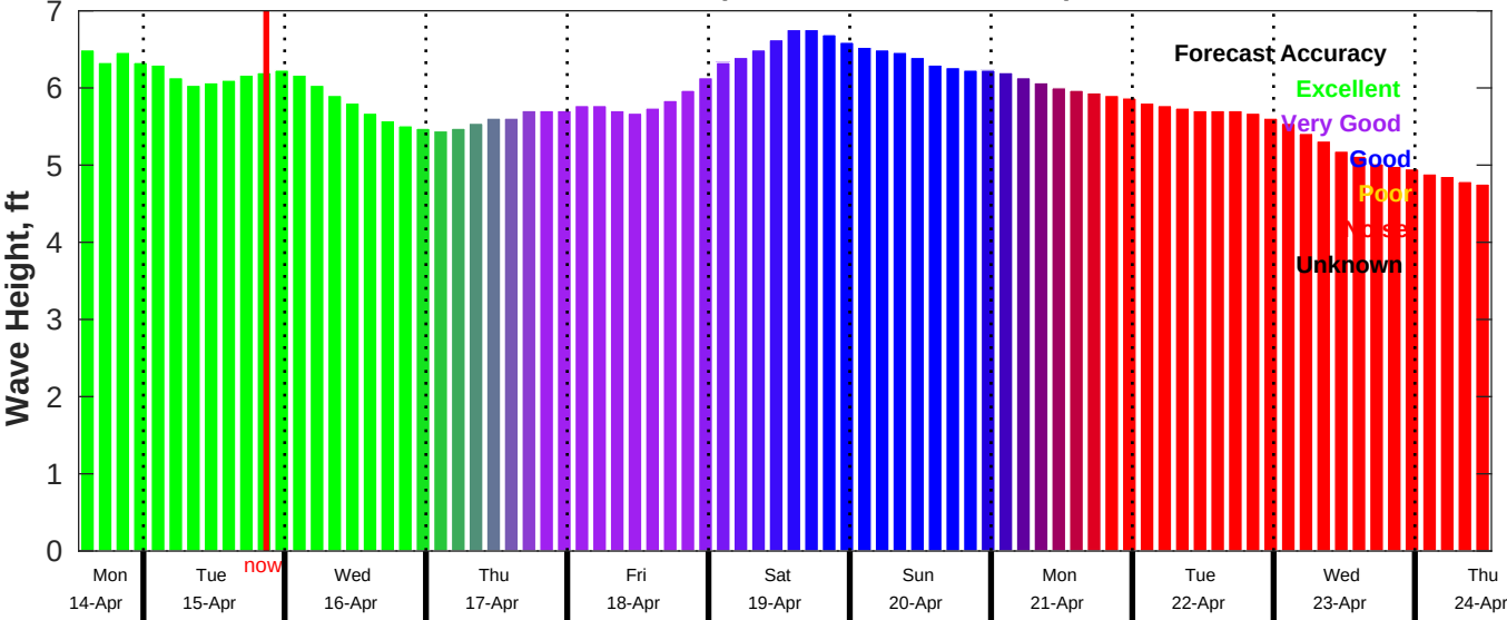
CMEMS Wave Forecast for NDBC 51209 from 14-Apr-2025 13:00:00 to 24-Apr-2025 13:00:00
