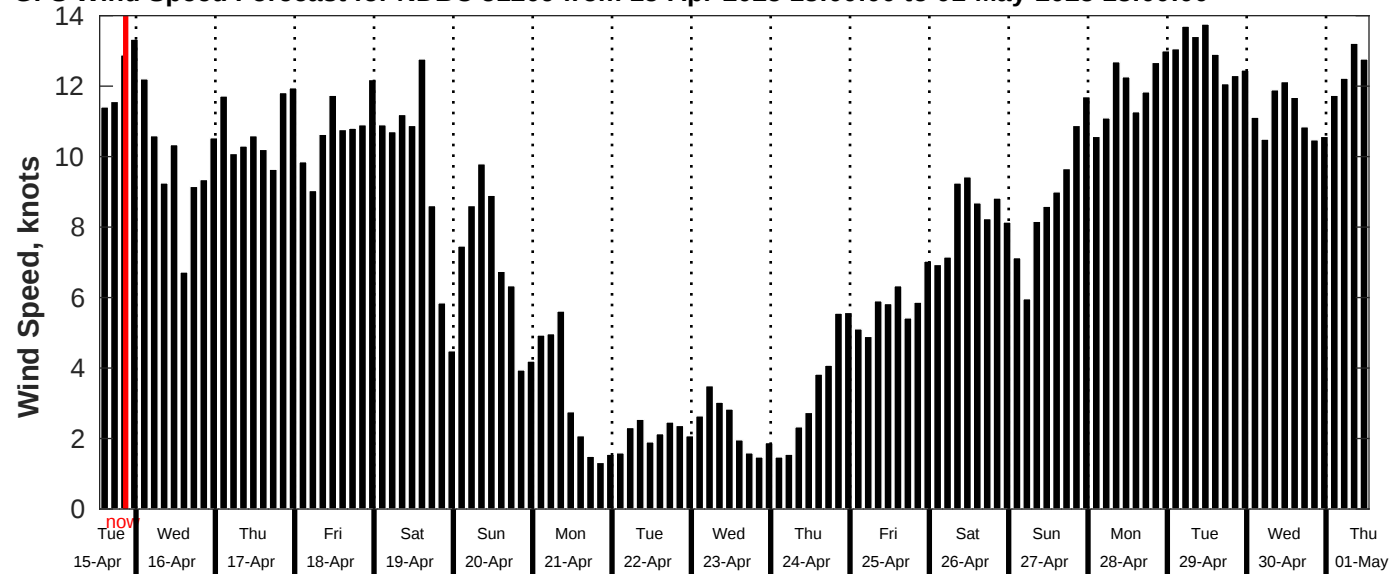
GFS Wind Speed Forecast for NDBC 51209 from 15-Apr-2025 13:00:00 to 01-May-2025 13:00:00
