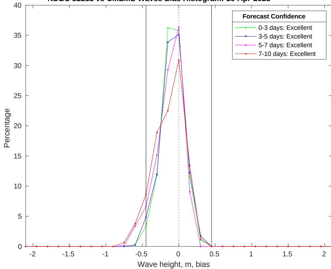
NDBC 52211 vs CMEMS Waves Bias Histogram: 16-Apr-2025
