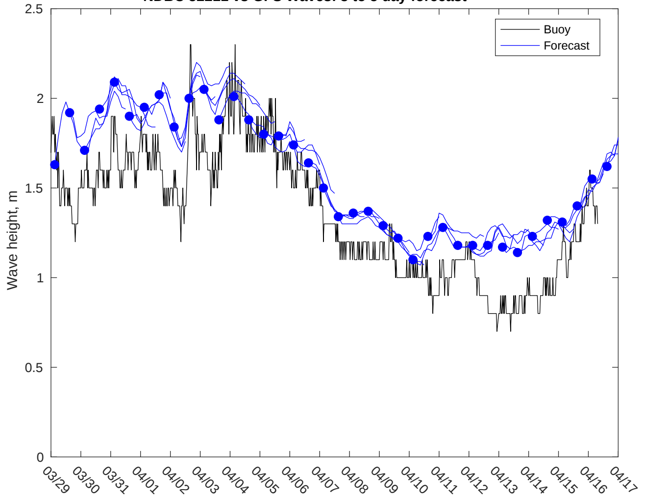
NDBC 52211 vs GFS Waves: 3 to 5 day forecast
