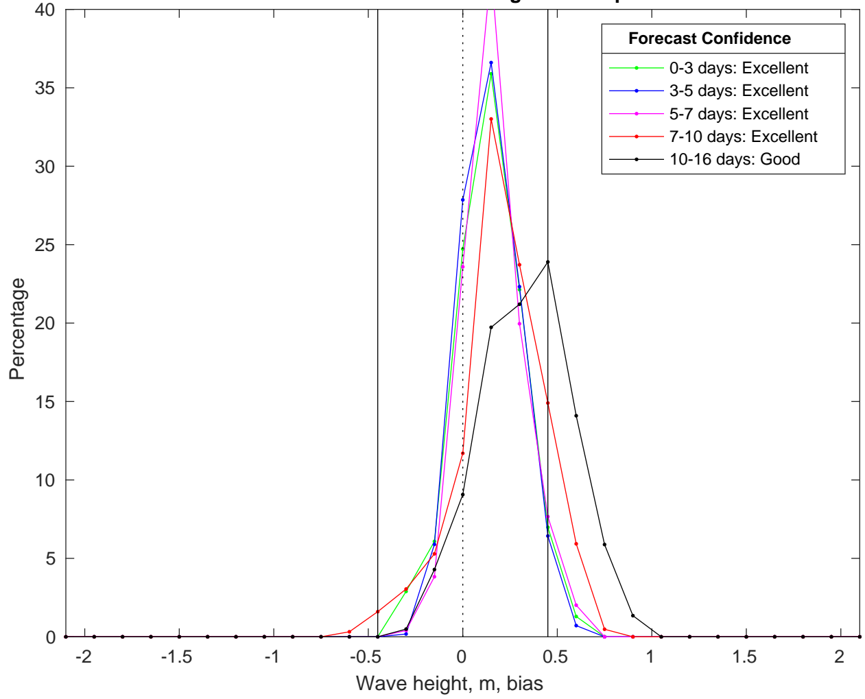
NDBC 52211 vs GFS Waves Bias Histogram: 16-Apr-2025
