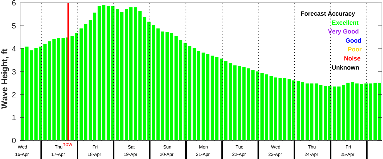
CMEMS Wave Forecast for NDBC 52211 from 15-Apr-2025 10:00:00 to 25-Apr-2025 10:00:00
