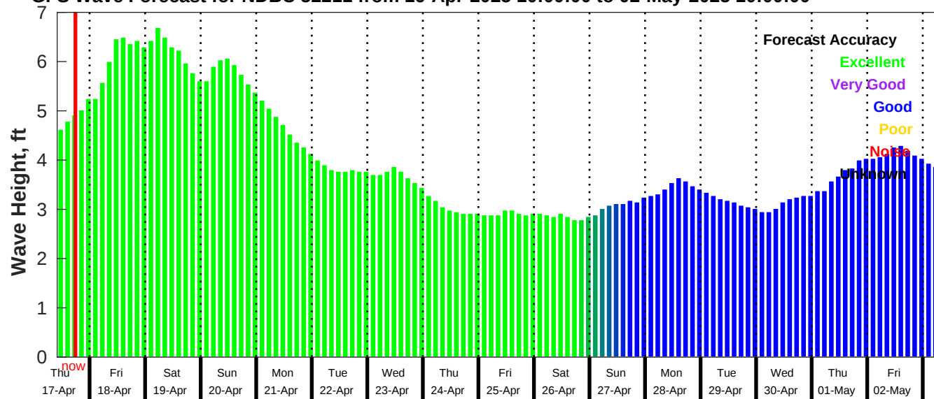
GFS Wave Forecast for NDBC 52211 from 16-Apr-2025 10:00:00 to 02-May-2025 10:00:00
