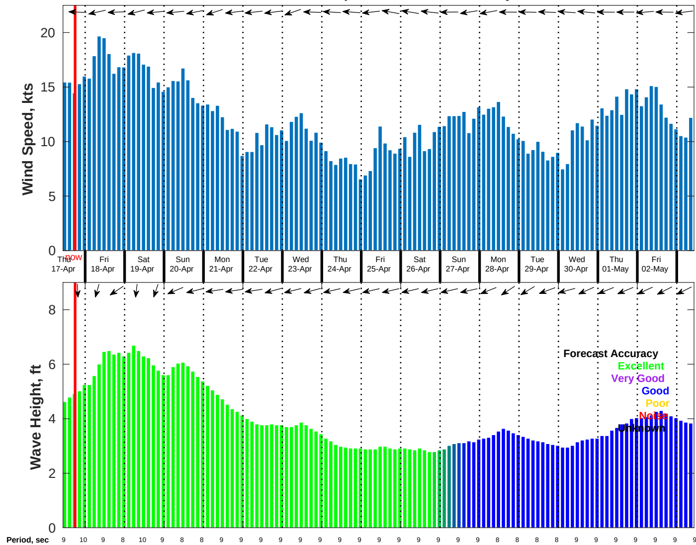
Wind & Wave Forecast for NDBC 52211 from 16-Apr-2025 10:00:00 to 02-May-2025 10:00:00
