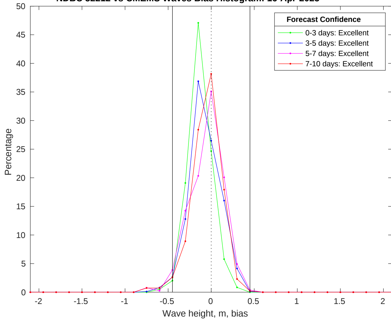
NDBC 52212 vs CMEMS Waves Bias Histogram: 16-Apr-2025
