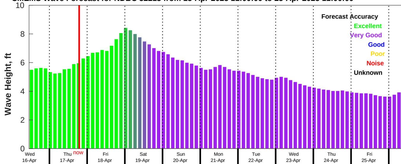
CMEMS Wave Forecast for NDBC 52213 from 15-Apr-2025 11:00:00 to 25-Apr-2025 11:00:00
