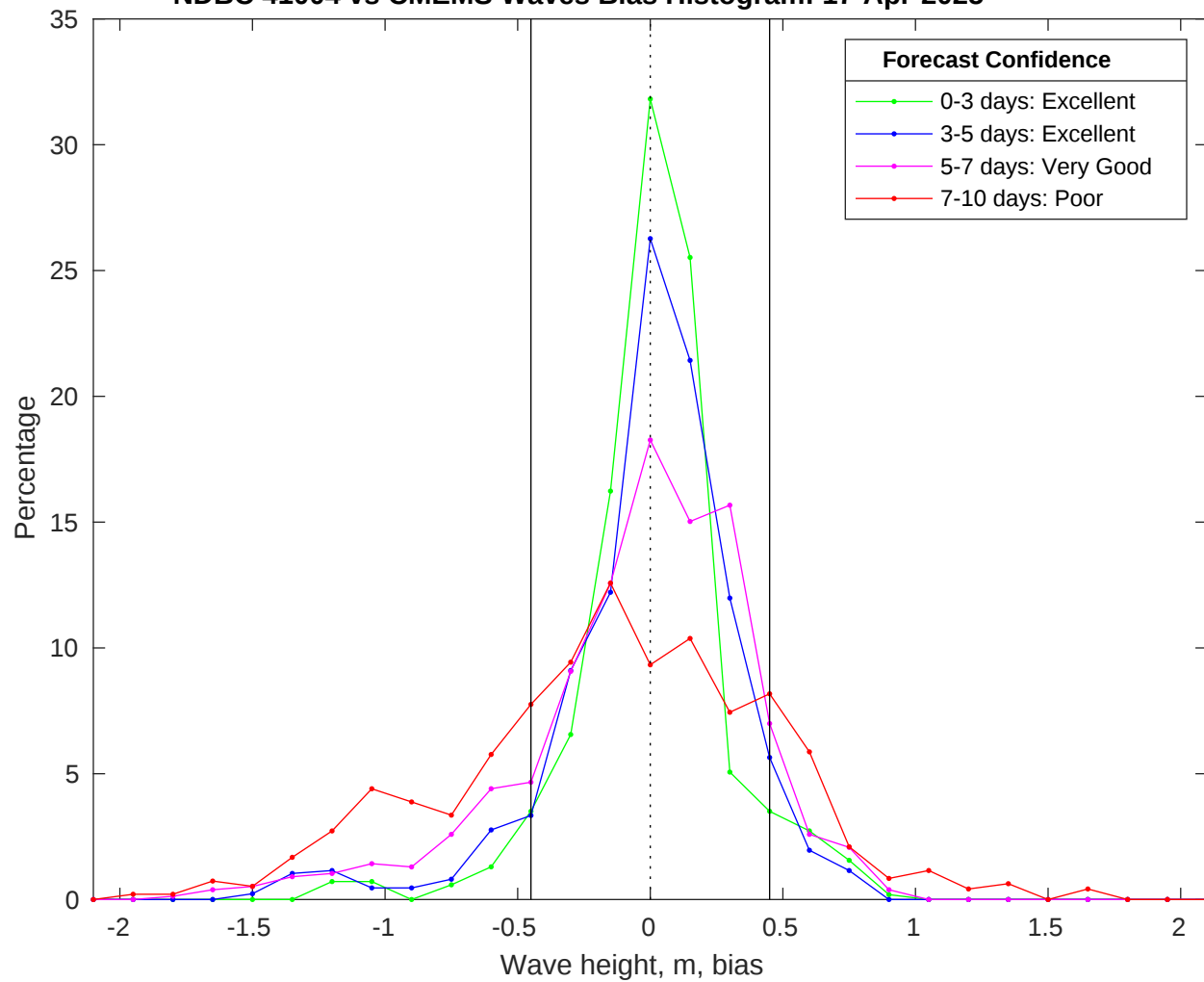
NDBC 41004 vs CMEMS Waves Bias Histogram: 17-Apr-2025
