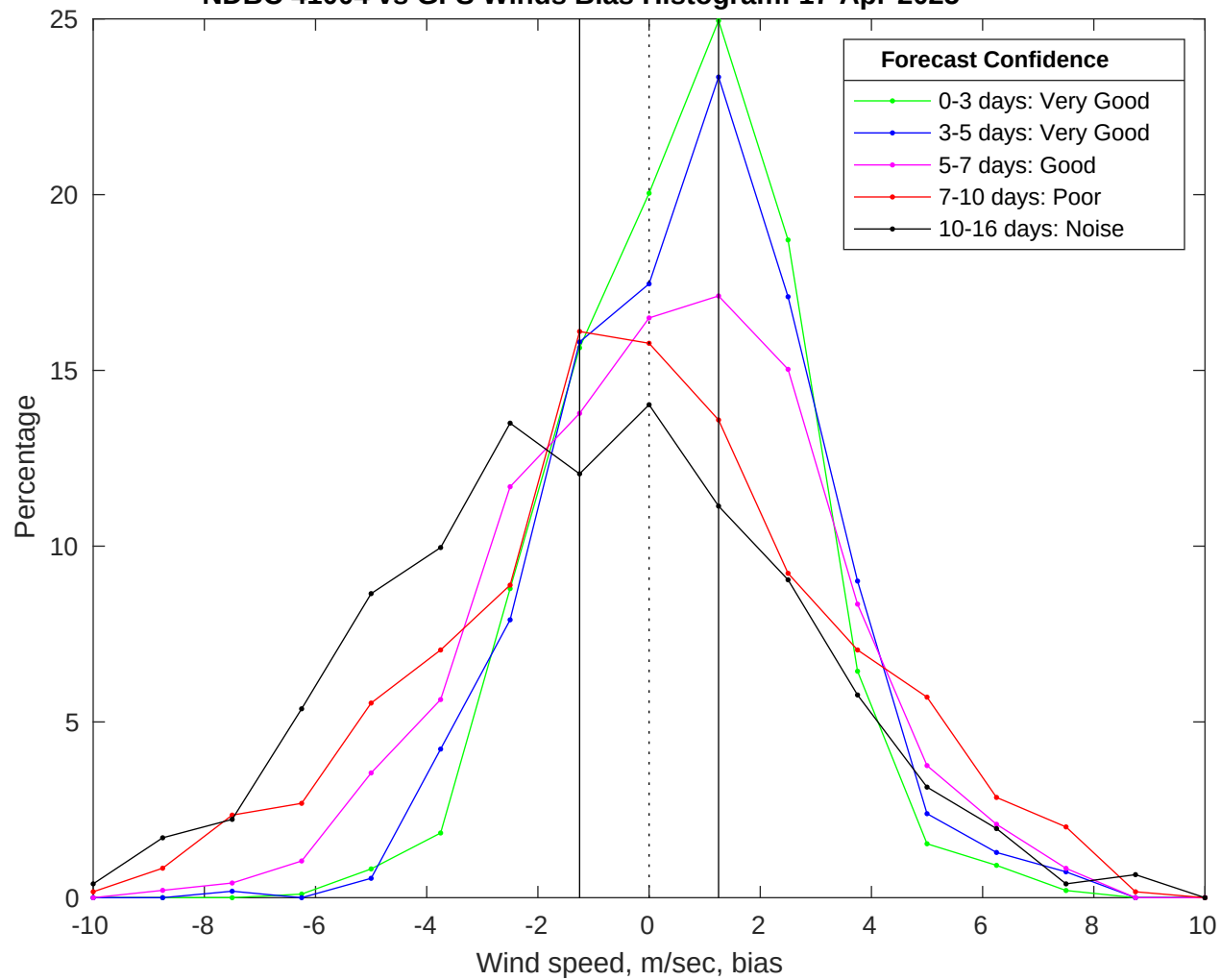
NDBC 41004 vs GFS Winds Bias Histogram: 17-Apr-2025
