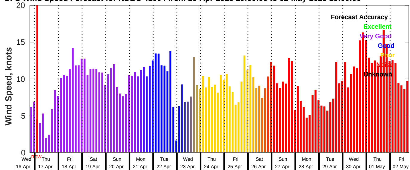
GFS Wind Speed Forecast for NDBC 41004 from 16-Apr-2025 19:00:00 to 02-May-2025 19:00:00
