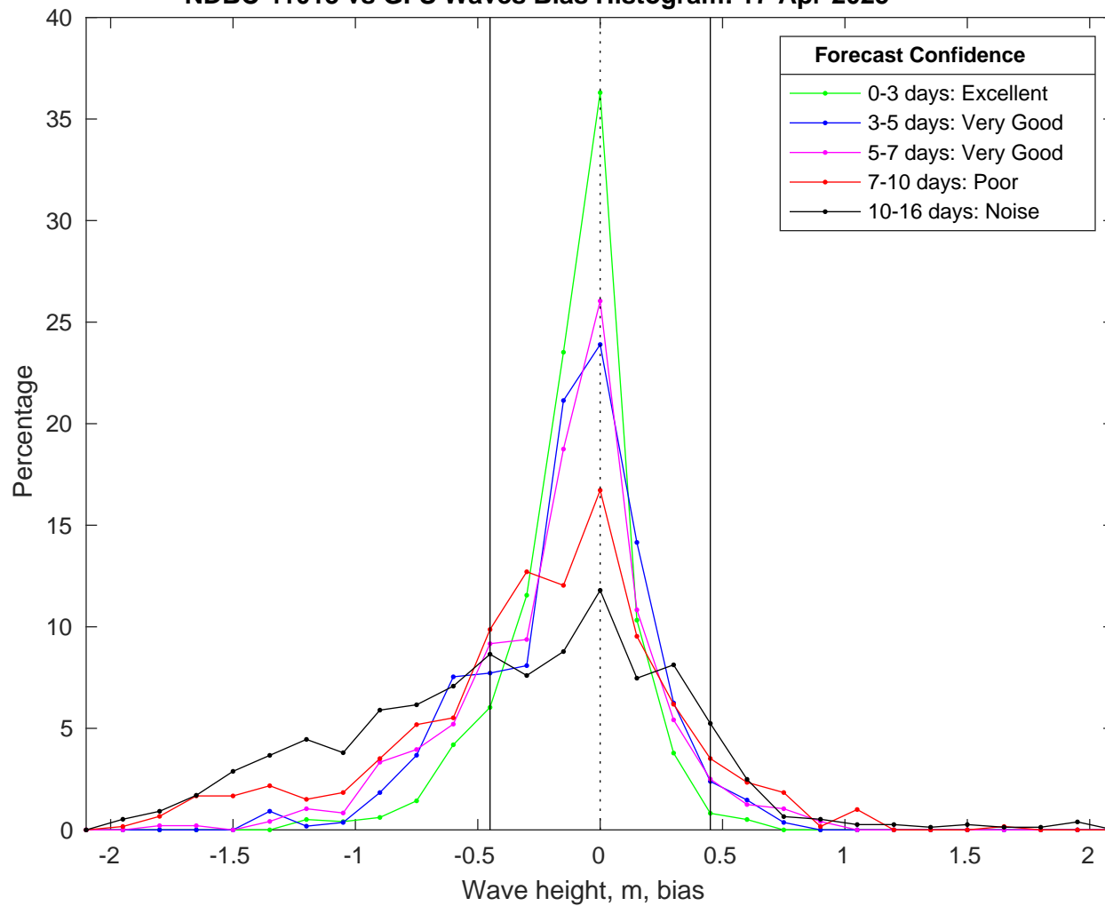
NDBC 41013 vs GFS Waves Bias Histogram: 17-Apr-2025
