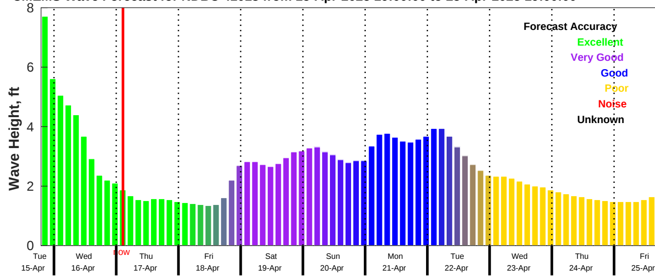
CMEMS Wave Forecast for NDBC 41013 from 15-Apr-2025 19:00:00 to 25-Apr-2025 19:00:00
