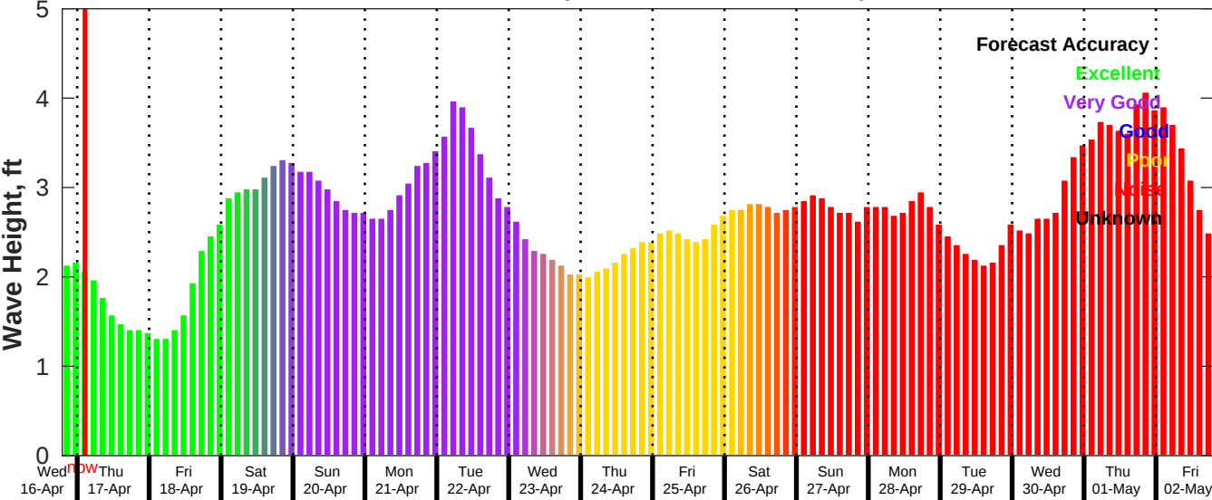
GFS Wave Forecast for NDBC 41013 from 16-Apr-2025 19:00:00 to 02-May-2025 19:00:00
