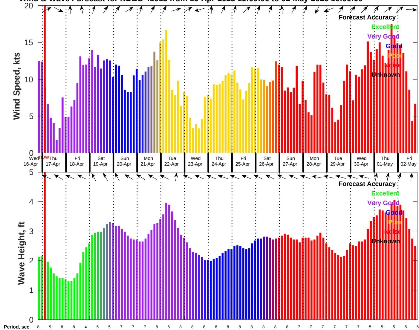
Wind & Wave Forecast for NDBC 41013 from 16-Apr-2025 19:00:00 to 02-May-2025 19:00:00
