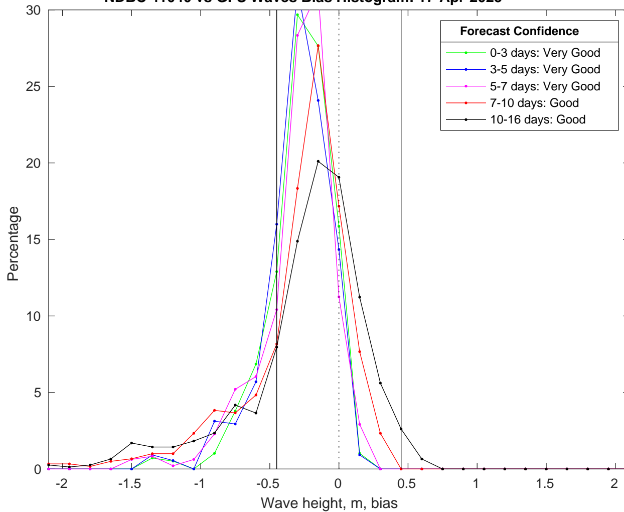
NDBC 41040 vs GFS Waves Bias Histogram: 17-Apr-2025
