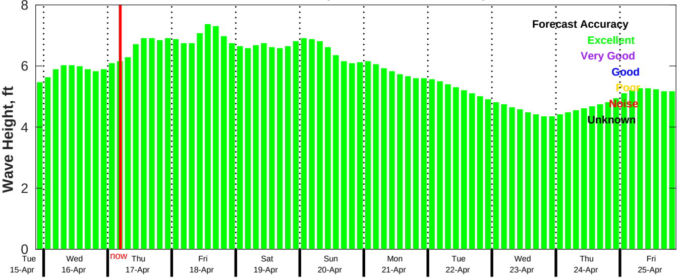
CMEMS Wave Forecast for NDBC 41040 from 15-Apr-2025 21:00:00 to 25-Apr-2025 21:00:00
