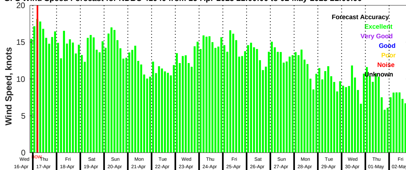
GFS Wind Speed Forecast for NDBC 41040 from 16-Apr-2025 21:00:00 to 02-May-2025 21:00:00
