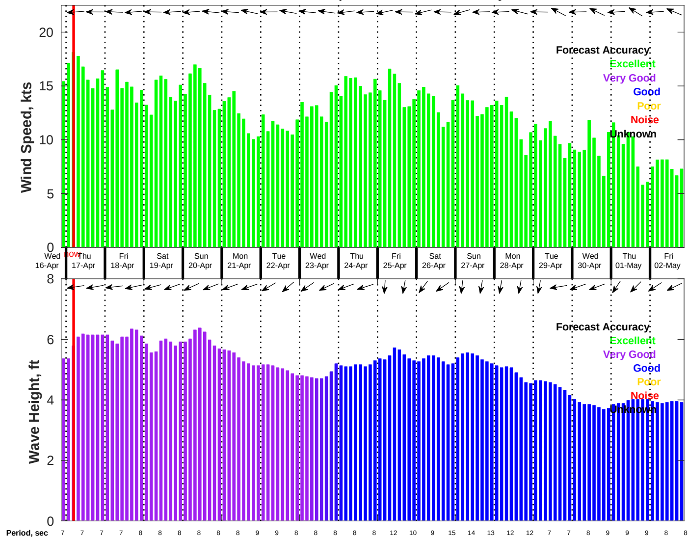
Wind & Wave Forecast for NDBC 41040 from 16-Apr-2025 21:00:00 to 02-May-2025 21:00:00
