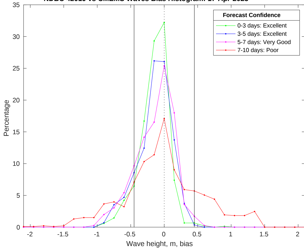
NDBC 42019 vs CMEMS Waves Bias Histogram: 17-Apr-2025
