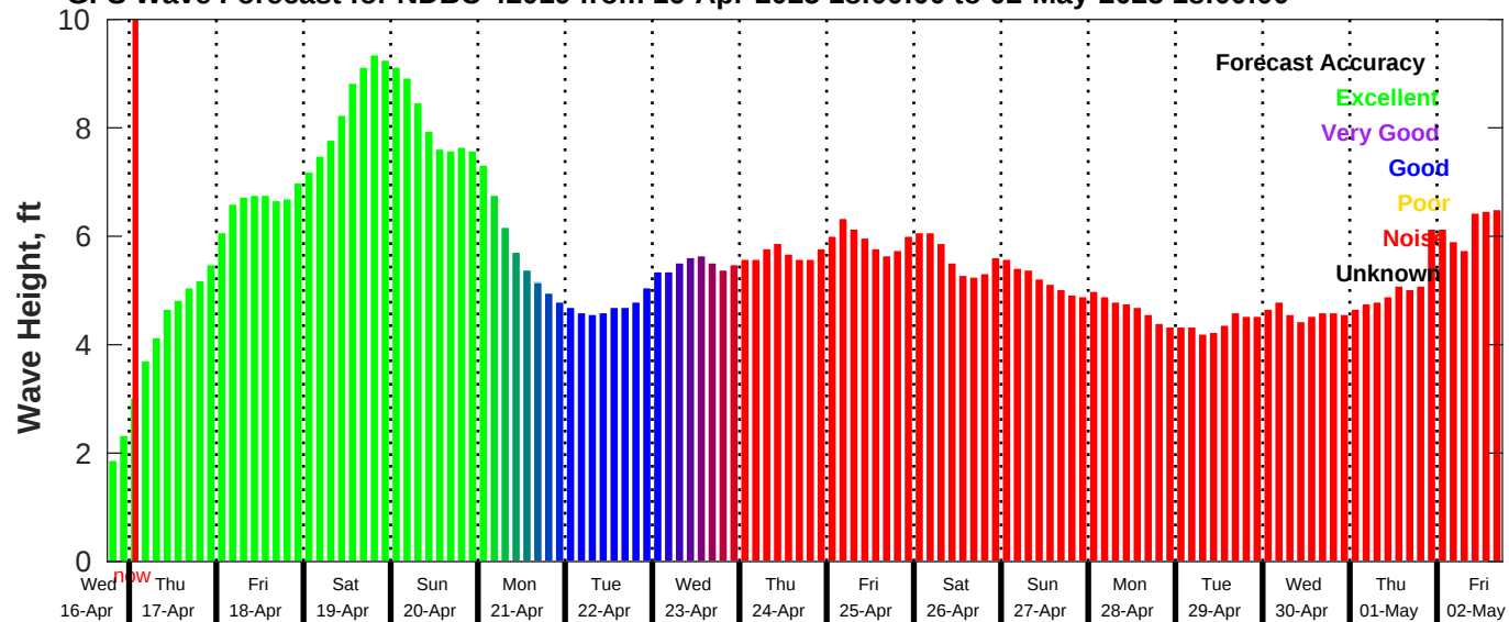
GFS Wave Forecast for NDBC 42019 from 16-Apr-2025 18:00:00 to 02-May-2025 18:00:00
