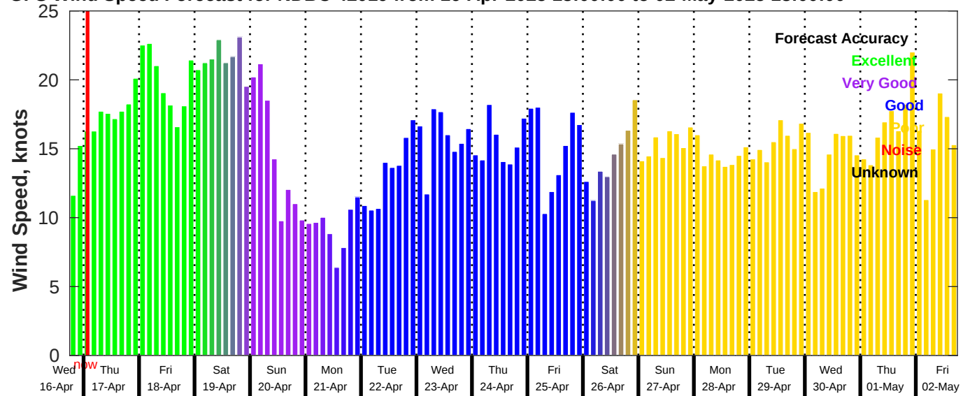
GFS Wind Speed Forecast for NDBC 42019 from 16-Apr-2025 18:00:00 to 02-May-2025 18:00:00
