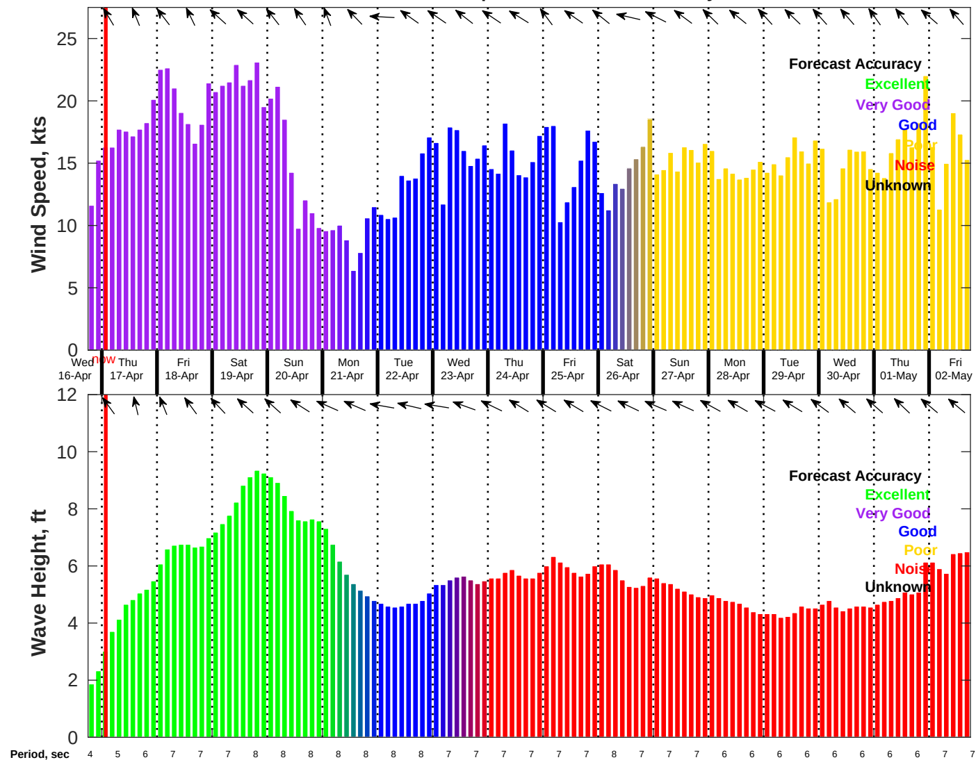
Wind & Wave Forecast for NDBC 42019 from 16-Apr-2025 18:00:00 to 02-May-2025 18:00:00
